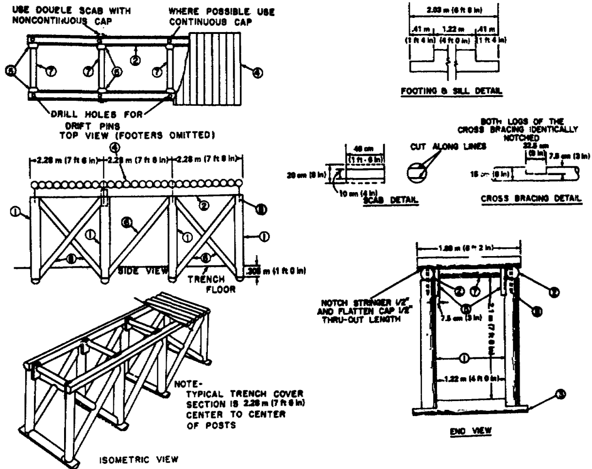
Figure 2-13. Trench section, log construction.
